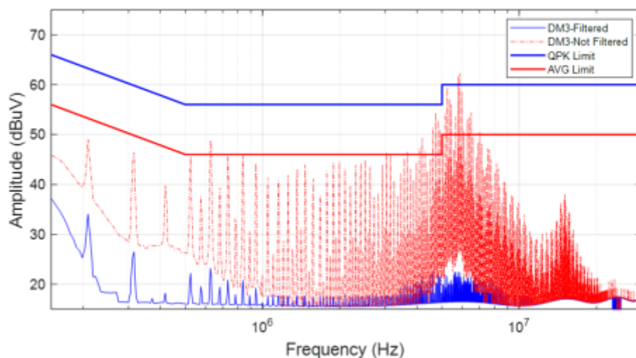
Figure 7. DM3 without (red) and with C_X capacitors (blue).
